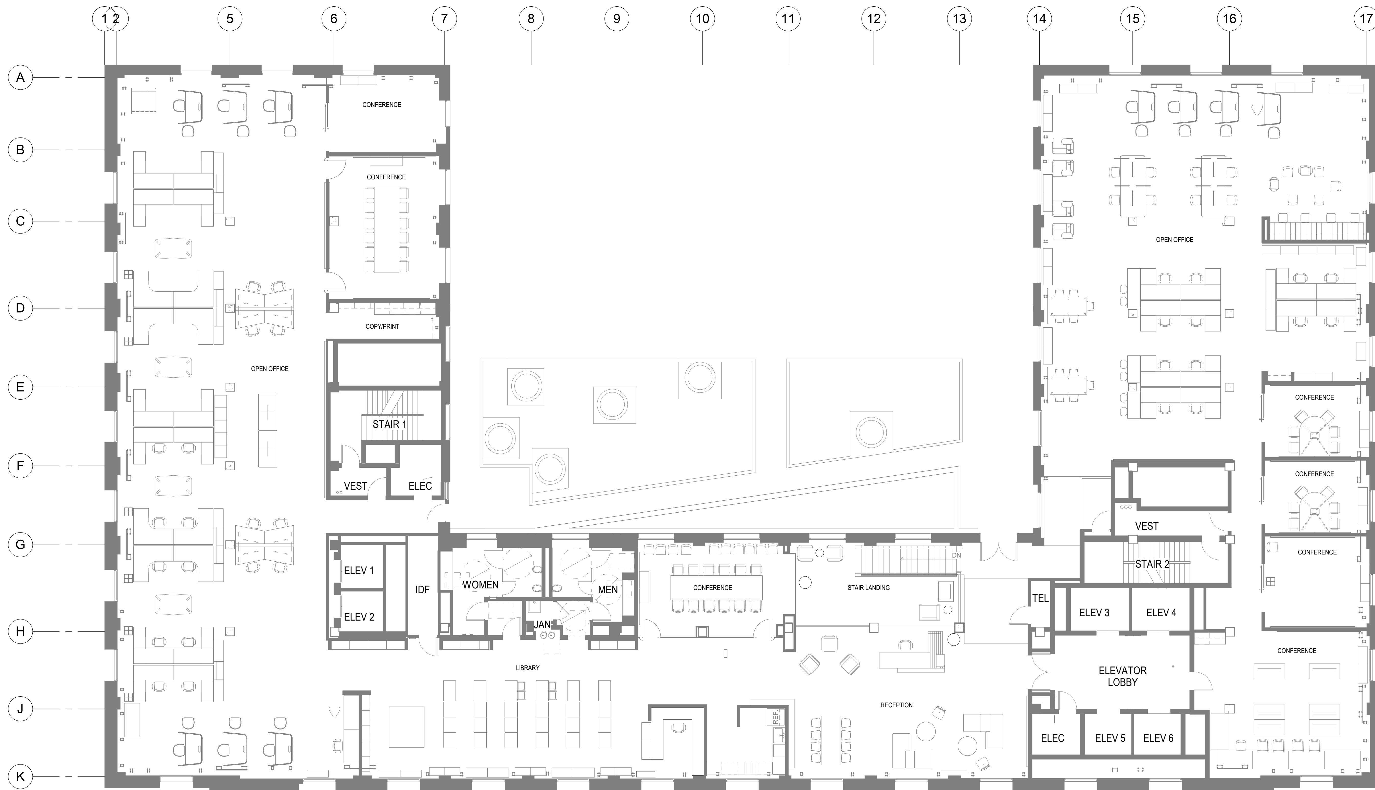
1 LEVEL 7 FLOOR EXISTING FURNITURE PLAN SCALE: 1/8" = 1'-0"
