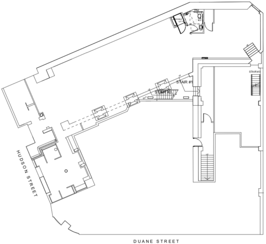
LOWER LEVEL
